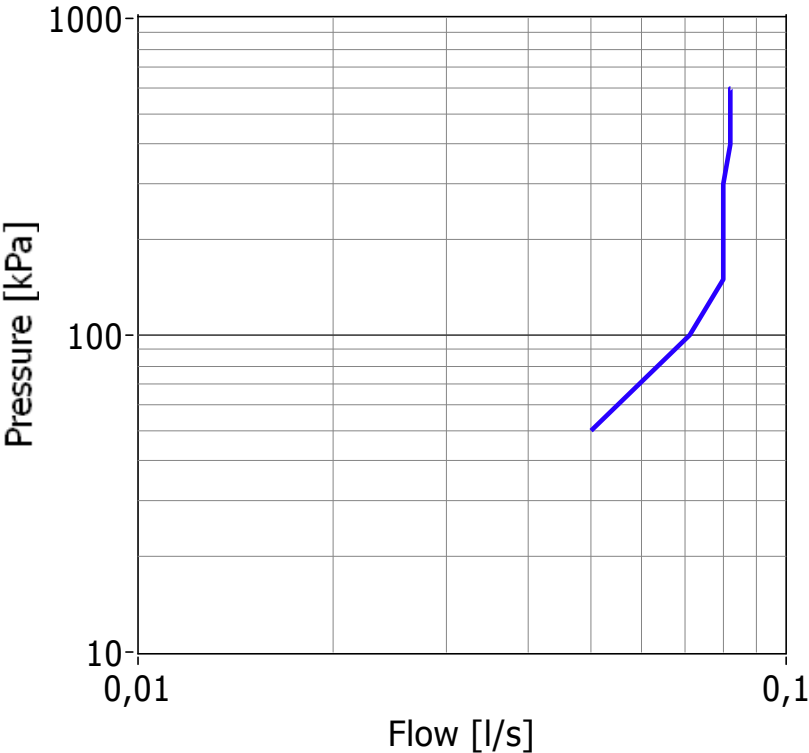
Pressure drop graph
