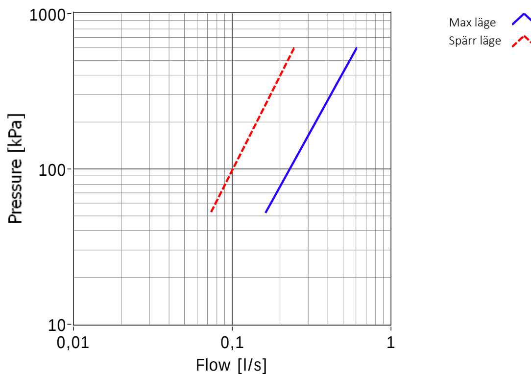
FLOW CHART AS A FUNCTION OF INLET PRESSURE
