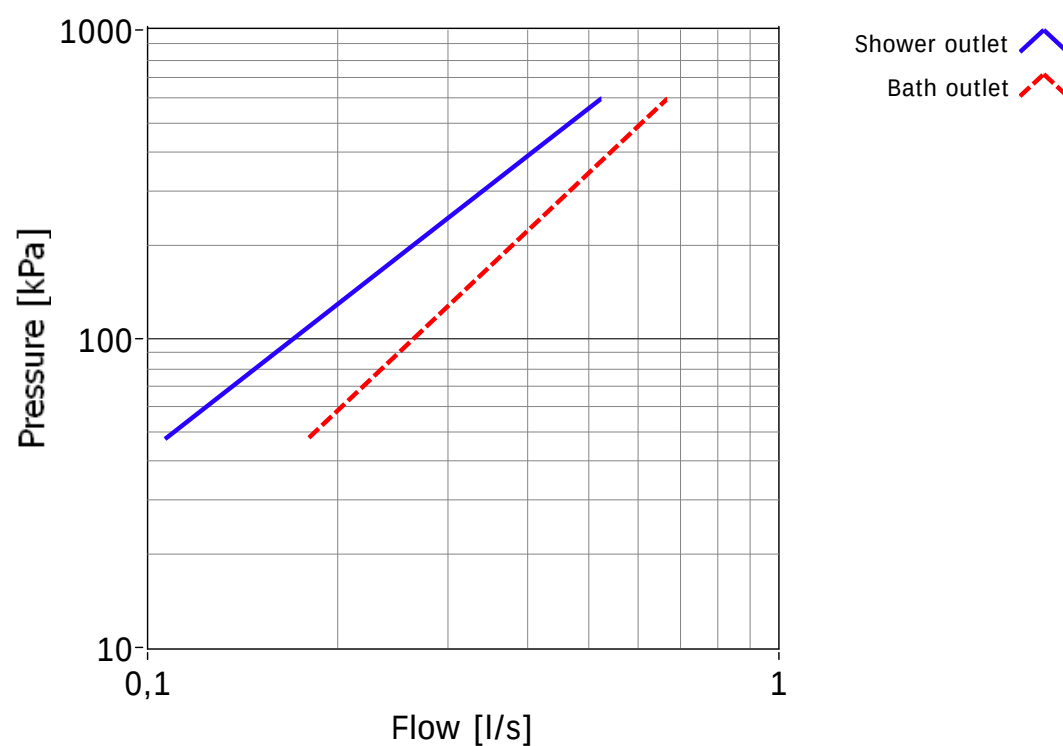
Pressure drop graph
